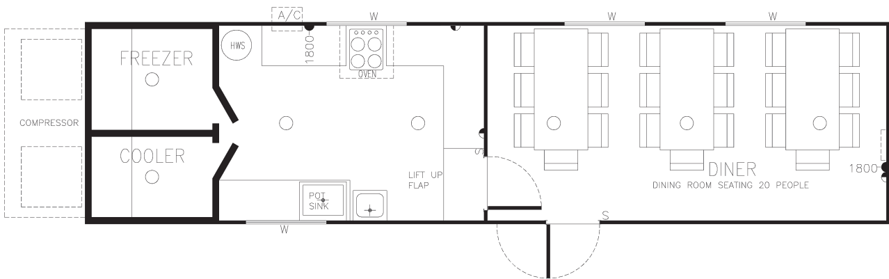
K-005 kitchen / diner 12.0 x 6.0m
