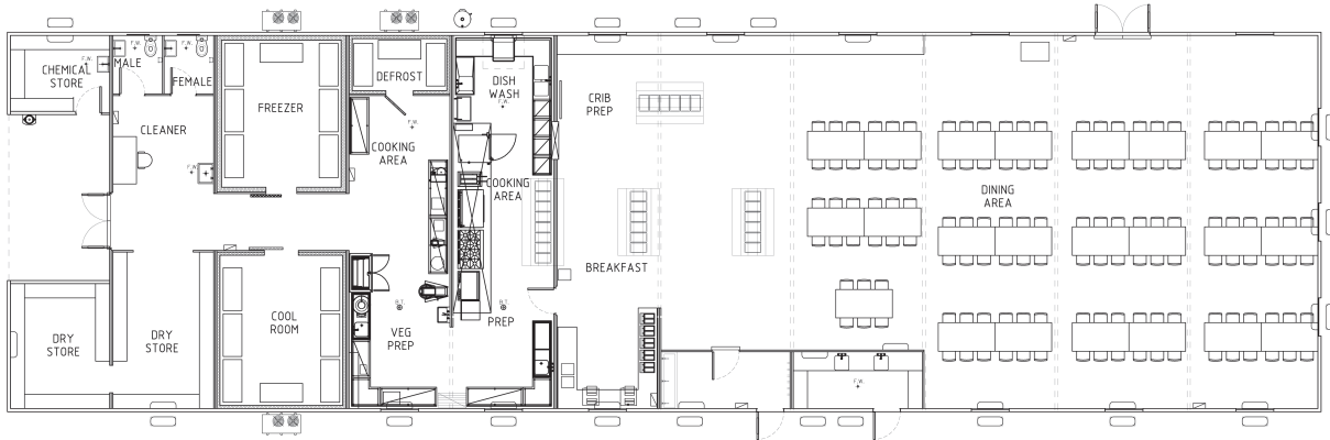
K-002 kitchen / diner 8.4 x 3.0m
