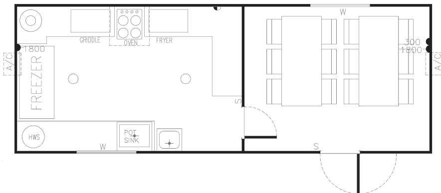
K-003 kitchen / diner 12.0 x 3.0m
