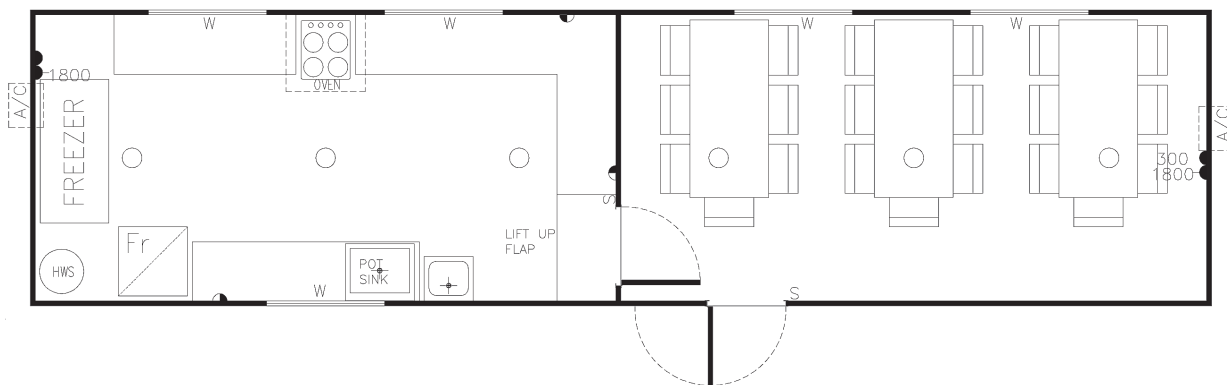
K-003 kitchen / diner 12.0 x 3.0m
